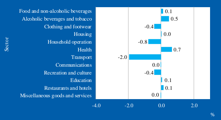
Figure 3: \Delta I per sector, July 2012
