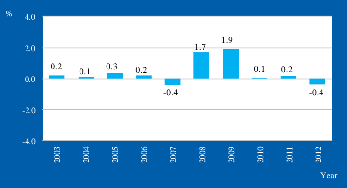
Figure 2: Monthly \Delta CPI for July, 2003 - 2012
