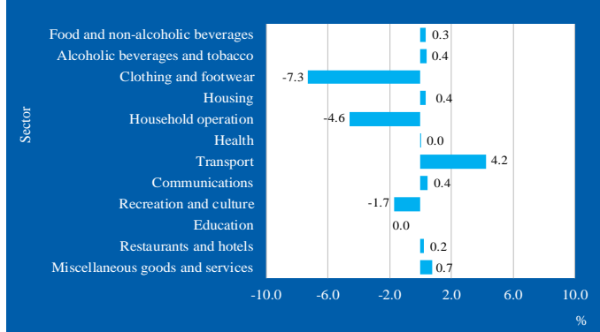
Figure 3: \Delta I per sector, April 2024
