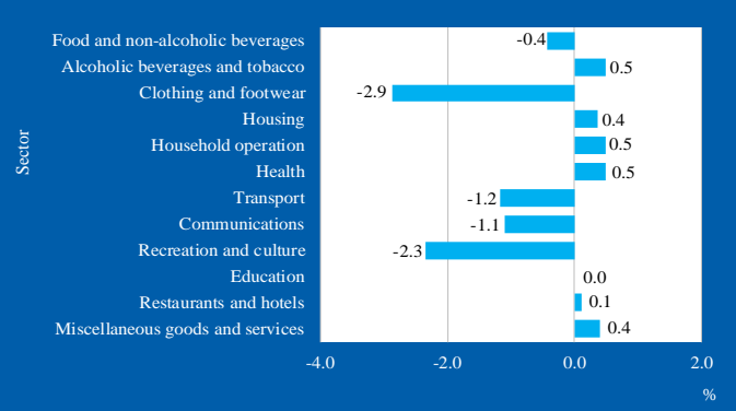
Figure 3: \Delta I per sector, June 2023
