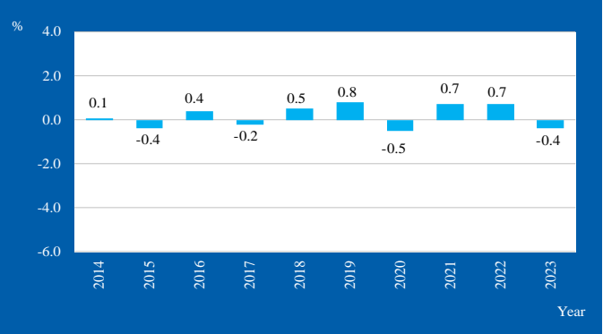
Figure 2: Monthly \Delta CPI for June, 2014 - 2023
