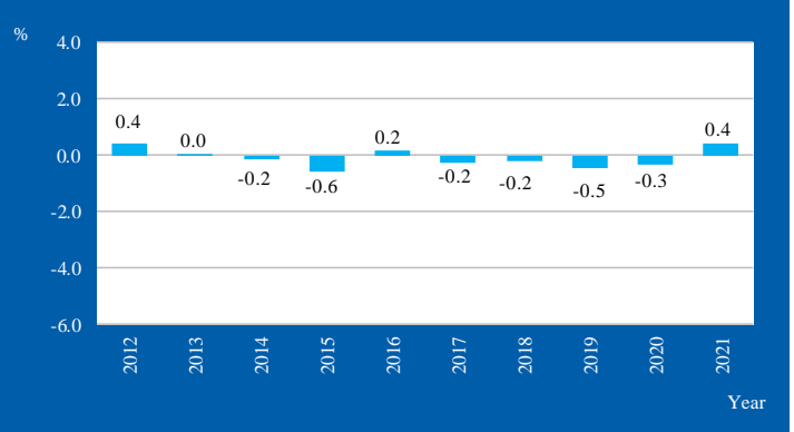
Figure 2: Monthly \Delta CPI for September, 2012 - 2021
