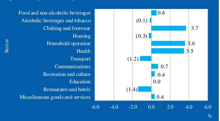
Figure 3: \Delta I per sector, September 2021
