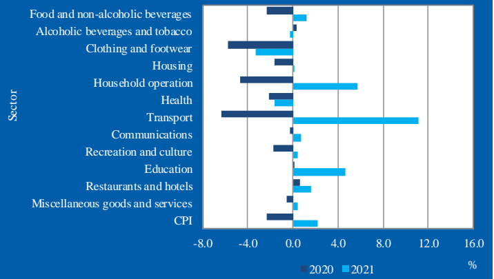
Figure 4: \Delta I per sector for September, 2020 - 2021
