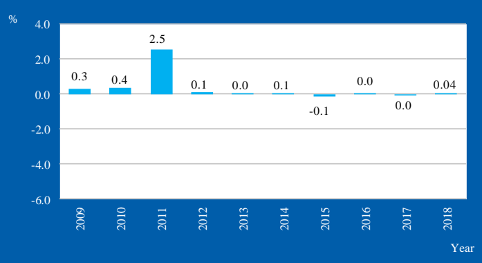
Figure 2: Monthly \Delta CPI for April, 2009 - 2018
