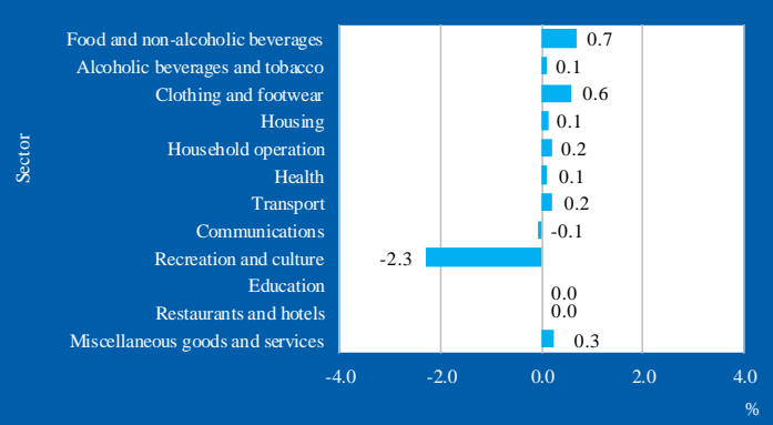
Figure 3: \Delta I per sector, April 2018
