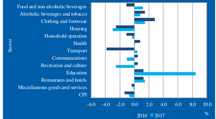
Figure 4: \Delta I per sector for August, 2016 - 2017
