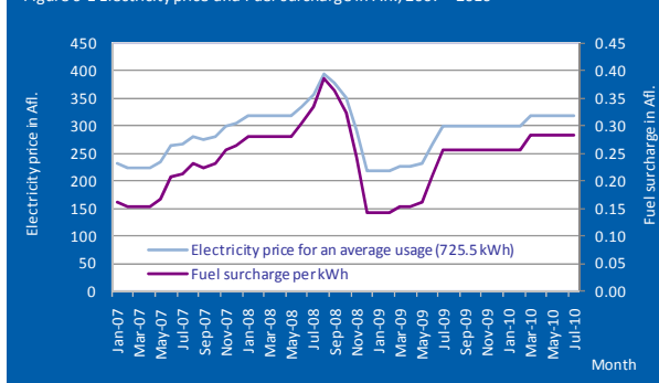
Figure 6-1 Electricity price and Fuel surcharge in Afl., 2007 - 2010
