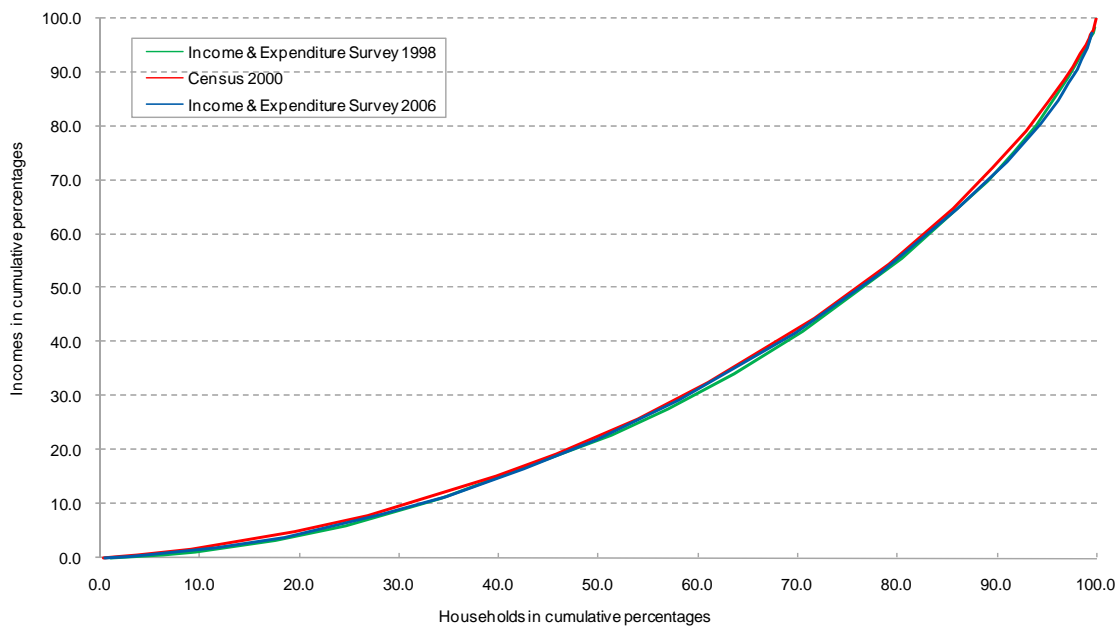
Figure 4. Lorenz curve based on Income and Expenditure Surveys 1998 and 2006 and Census 2000
